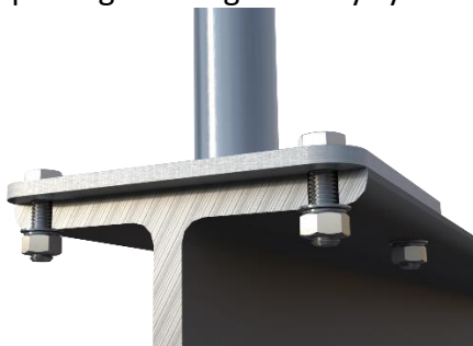
Steel Mounted Sectional Drawing
